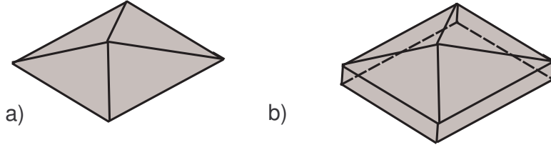
FIGURE 1. Pyramidal polyhedra
